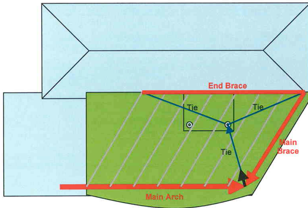
PLAN VIEW
